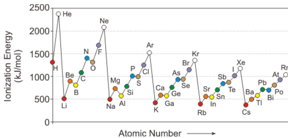
Figure: Ionization Energies
